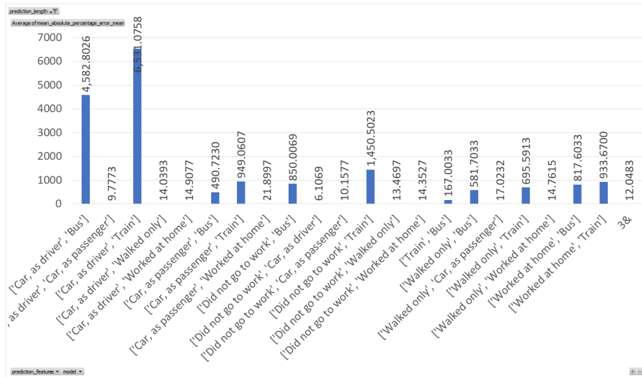
Fig. 2. Mean MAPE among all regressors in predicting two modes
